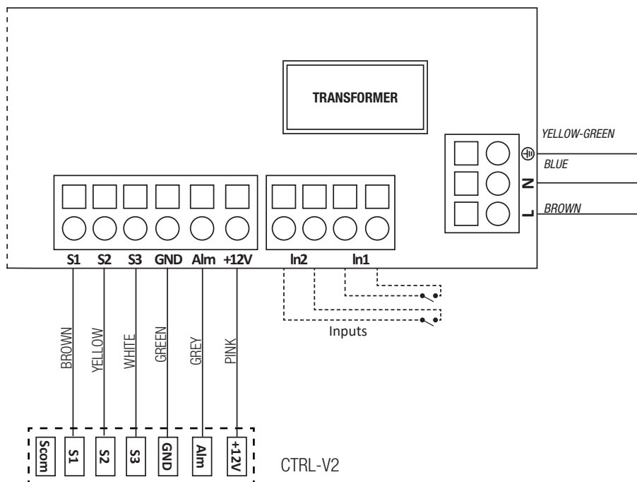
Fig. 5.m Electrical connections on the motherboard fitted in the terminal box.
