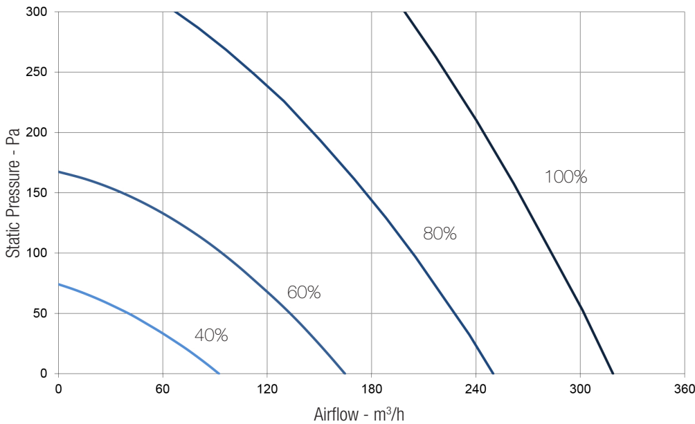
Fig. 6.b Intake curve according to Reg. 1253/2014 (ErP).
