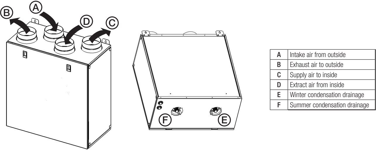
Fig. 3.a Connections
