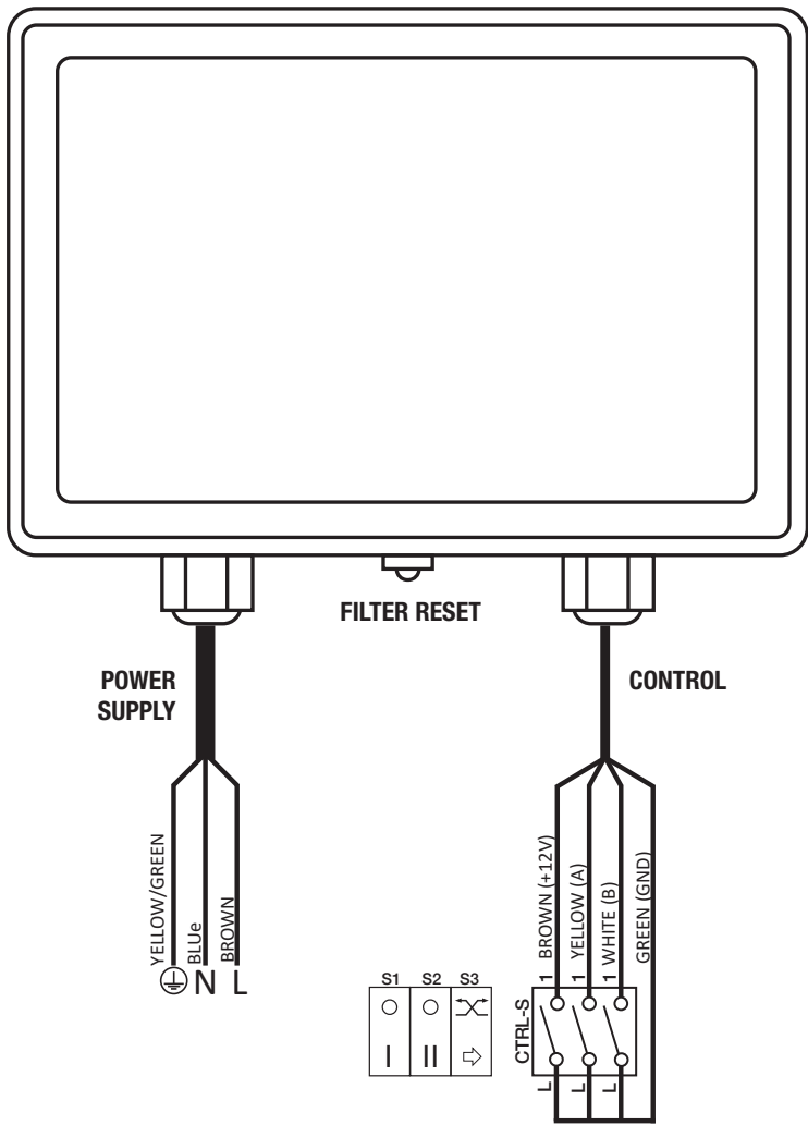
Fig. 5.f Electrical connection
