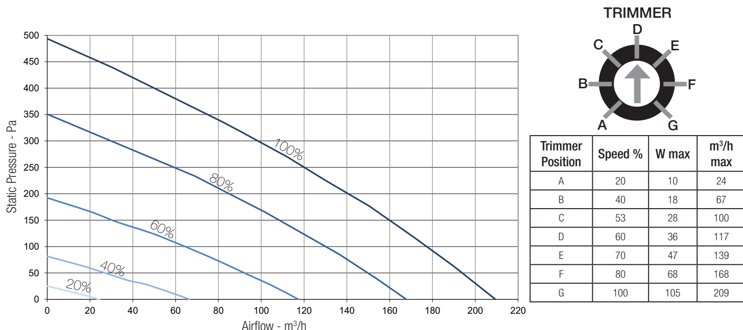
Fig. 6.a Intake curve according to Reg. 1253/2014 (ErP).
