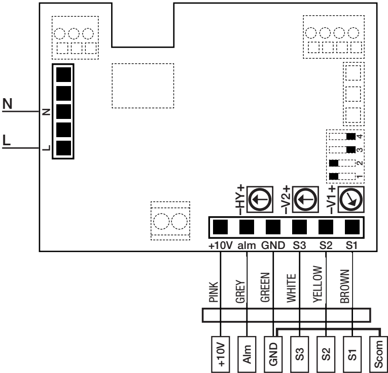
Fig. 5.q Electrical wirings on the motherboard on the machine.
